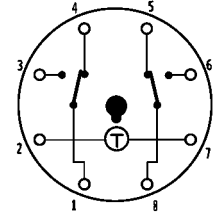
Bottom View of TDR
